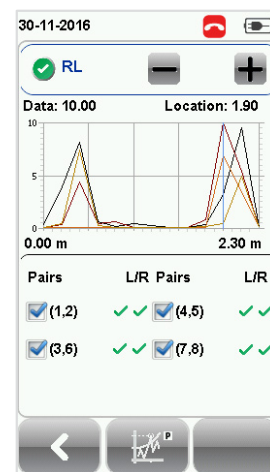
Return Loss Locator
