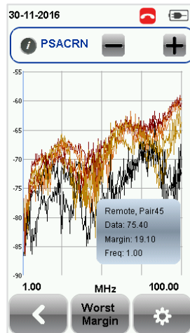
Power-sum ACRN (ISO only)
